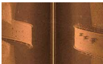
Ultra High-Definition SideVü (1200kHz)
